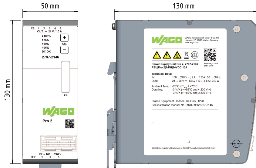
Figure 9: Dimensions
