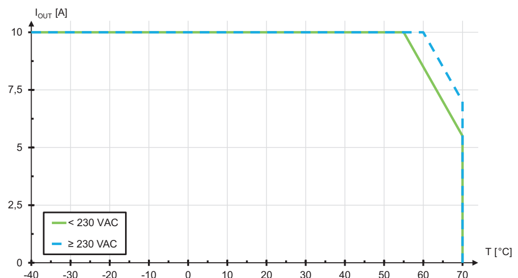
Figure 37: Derating (Temperature-Dependent)
