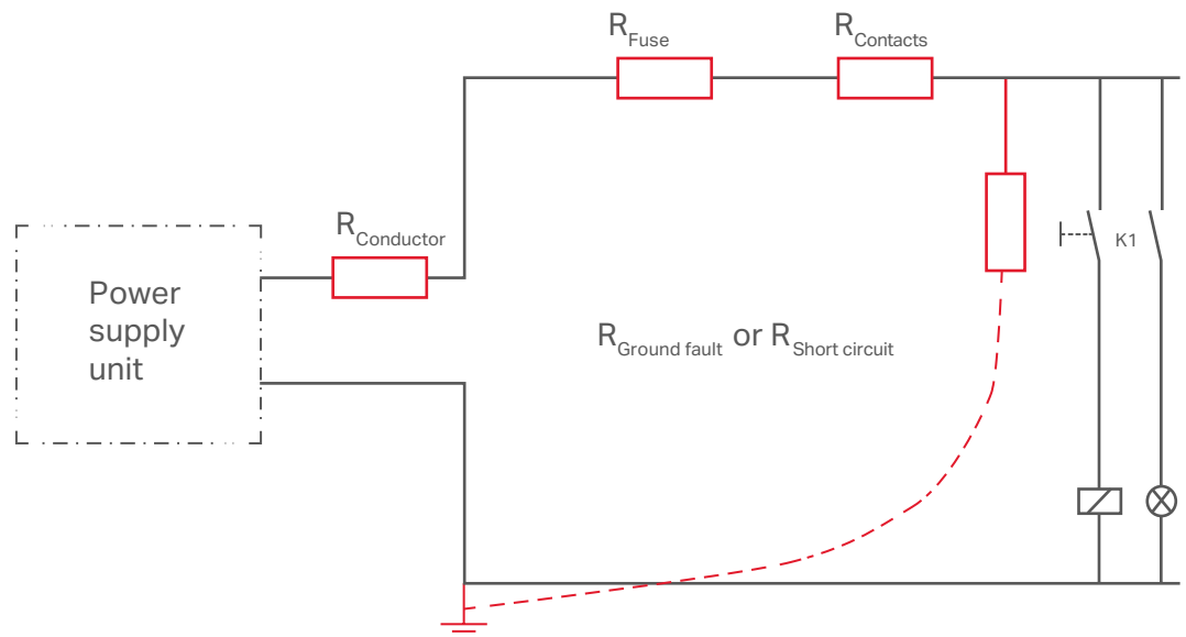
Figure 44: Loop Impedance
