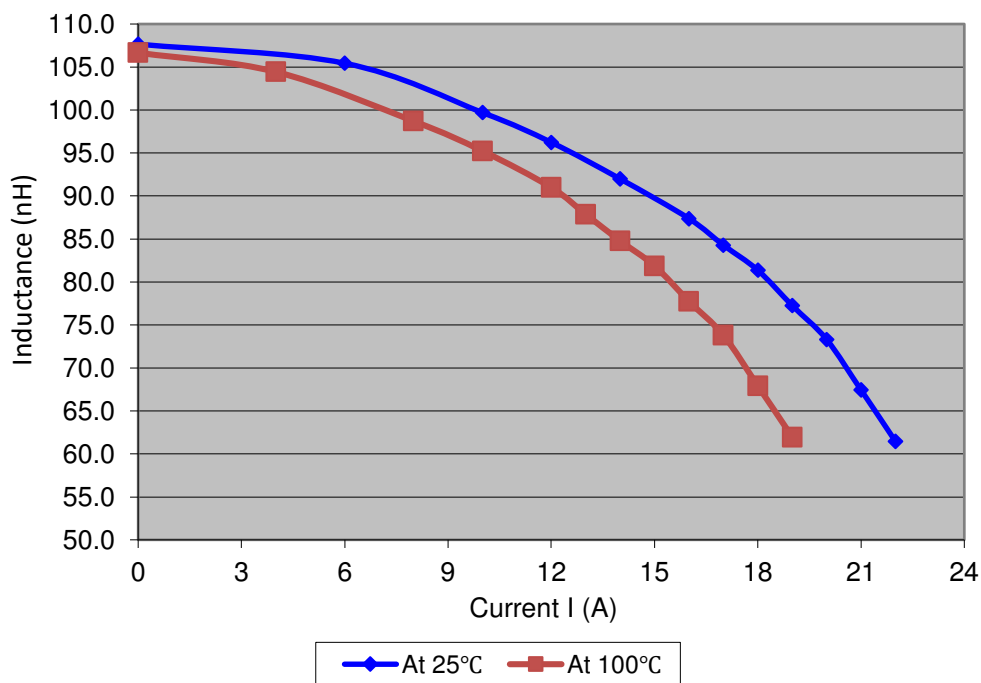
PG2289.101HLT, L vs I Curve
