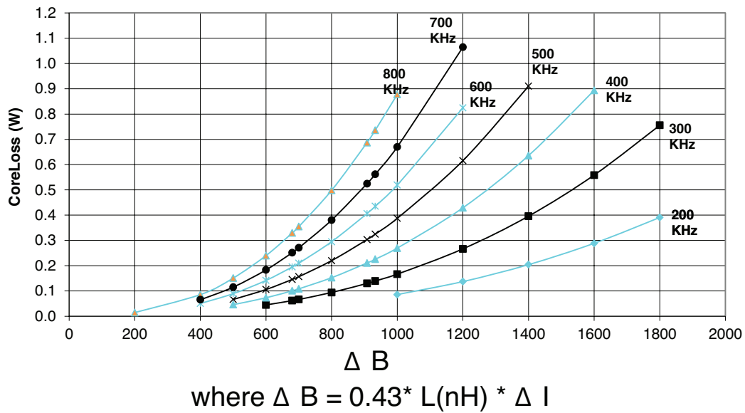
PGL6189.XXXHLT, Core Loss
