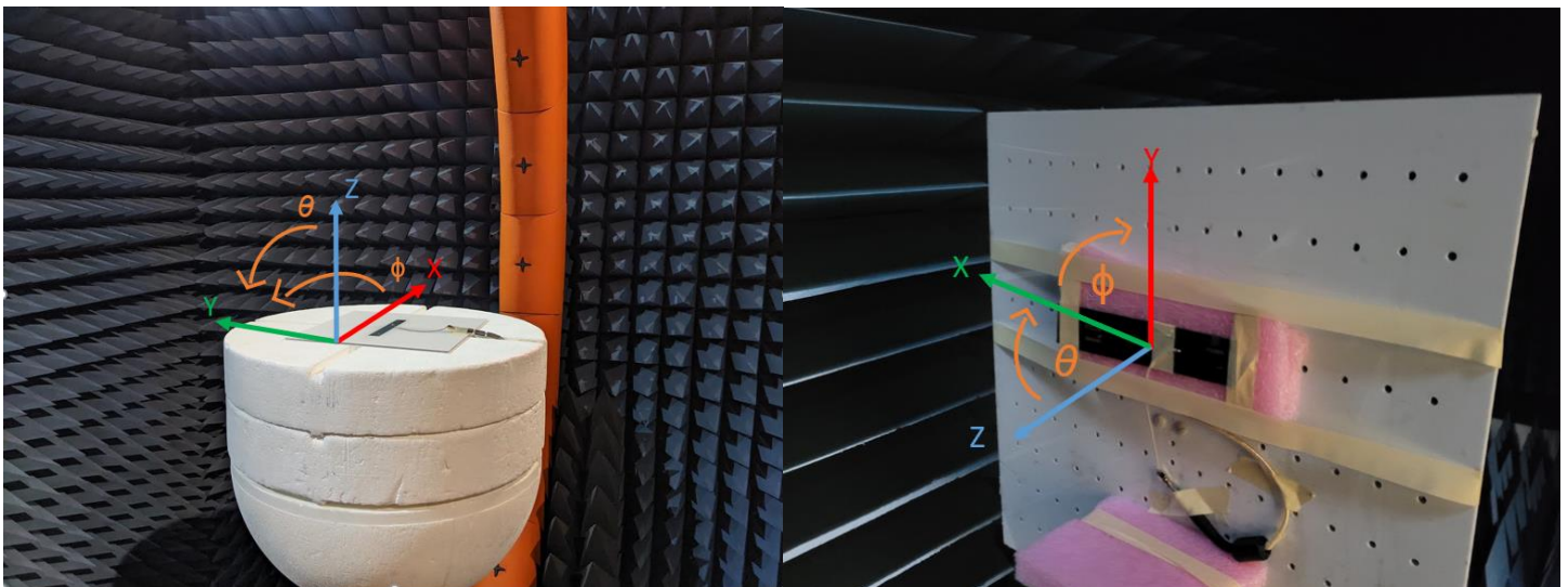
OTA Setup of the FXUB85.54.0150C in the SG24-L Satimo Test System For 600 MHz – 6 GHz Testing
