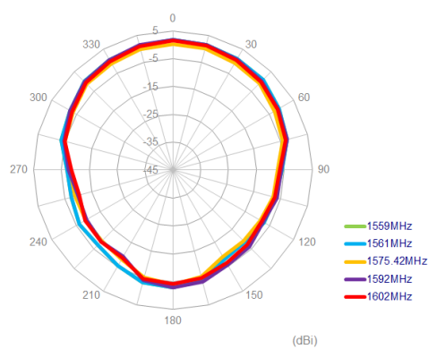
ZY Plane
