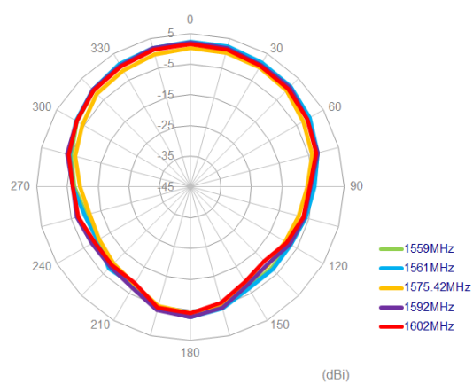
ZY Plane
