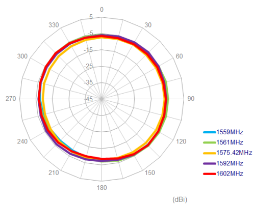
ZX Plane
