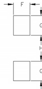
SUGGESTED PAD LAYOUT
