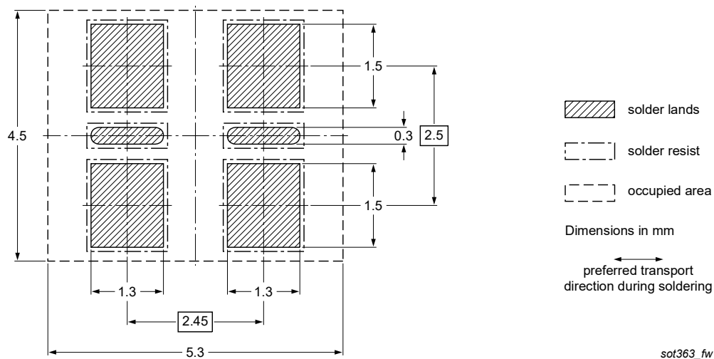
Fig. 13. Wave soldering footprint for TSSOP6 (SOT363)
