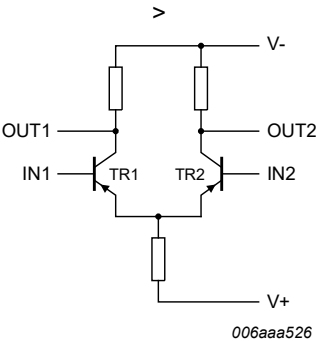
Fig. 10. Differential amplifier
