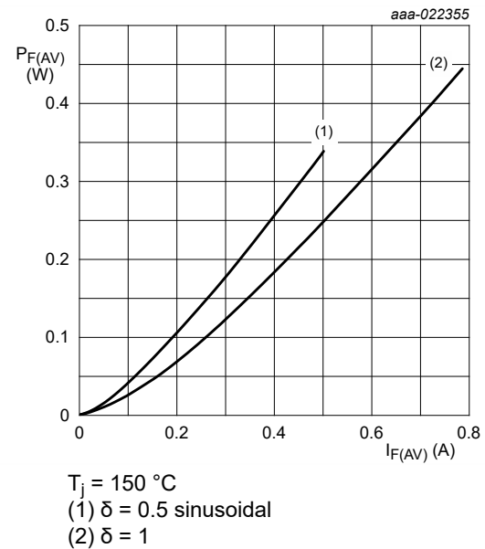
Fig. 6. Average forward power dissipation as a function of average forward current; typical values
