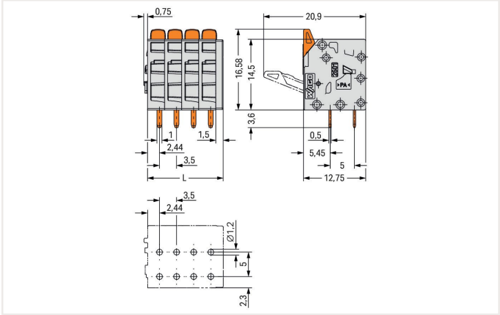
Dimensions in mm L = (pole no. – 1) x pin spacing + 5 mm
