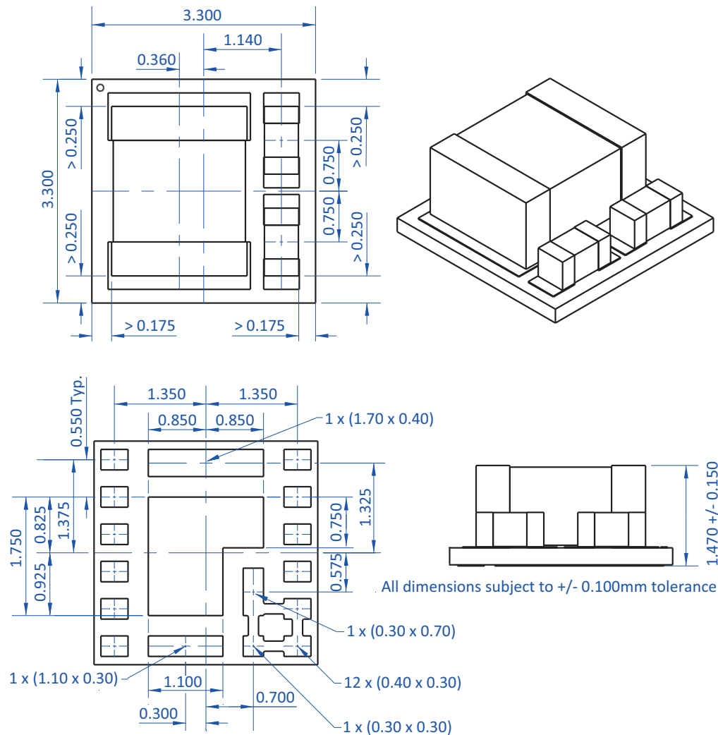
Figure 25 Dimensioned drawings
