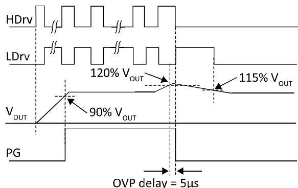
Figure 10 Illustration of latched OVP
