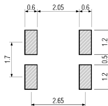
Figure 2) Land Pattern
