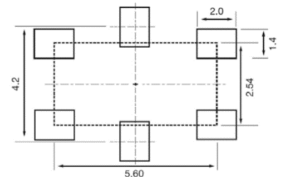
Figure 2) Land Pattern
