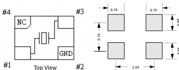
Figure 2) Suggested land pattern
