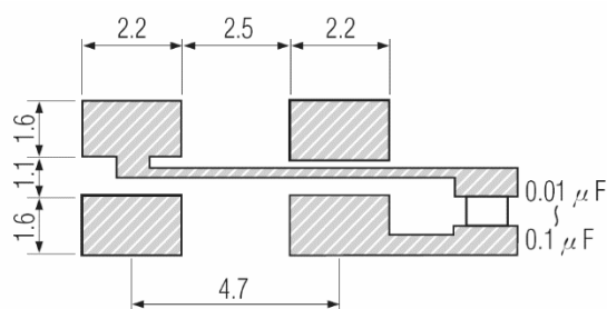
Figure 2) Land Pattern
