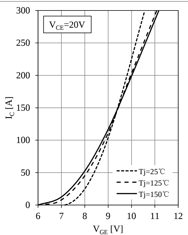
Fig 2. T1-T4 IGBT Transfer Characteristics
