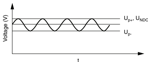
Non reversing recurrent waveform
