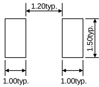
Recommended Pad Layout (mm)
