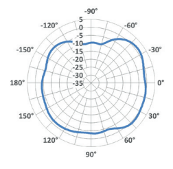
Vertical - 4000 MHz
