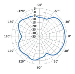
Vertical - 5500 MHz
