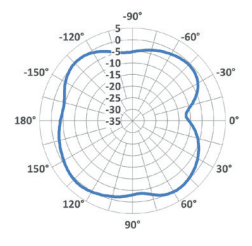
Vertical - 3500 MHz
