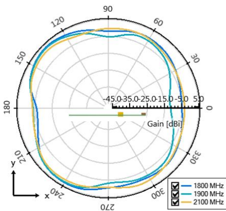
High Band measured at 1800, 1900, 850, 2100 MHz
