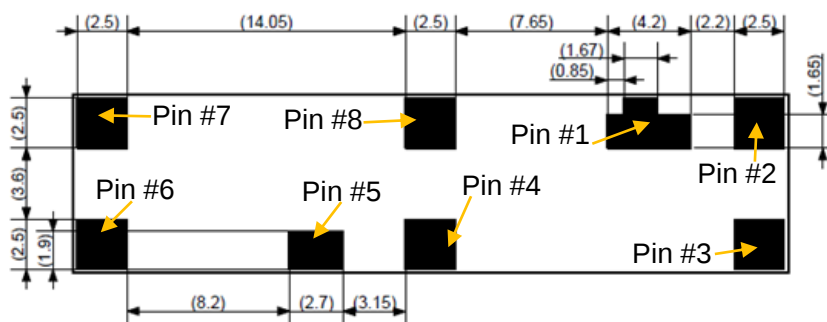
Bottom View
