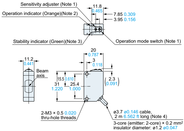
CX-41□ Sensor
