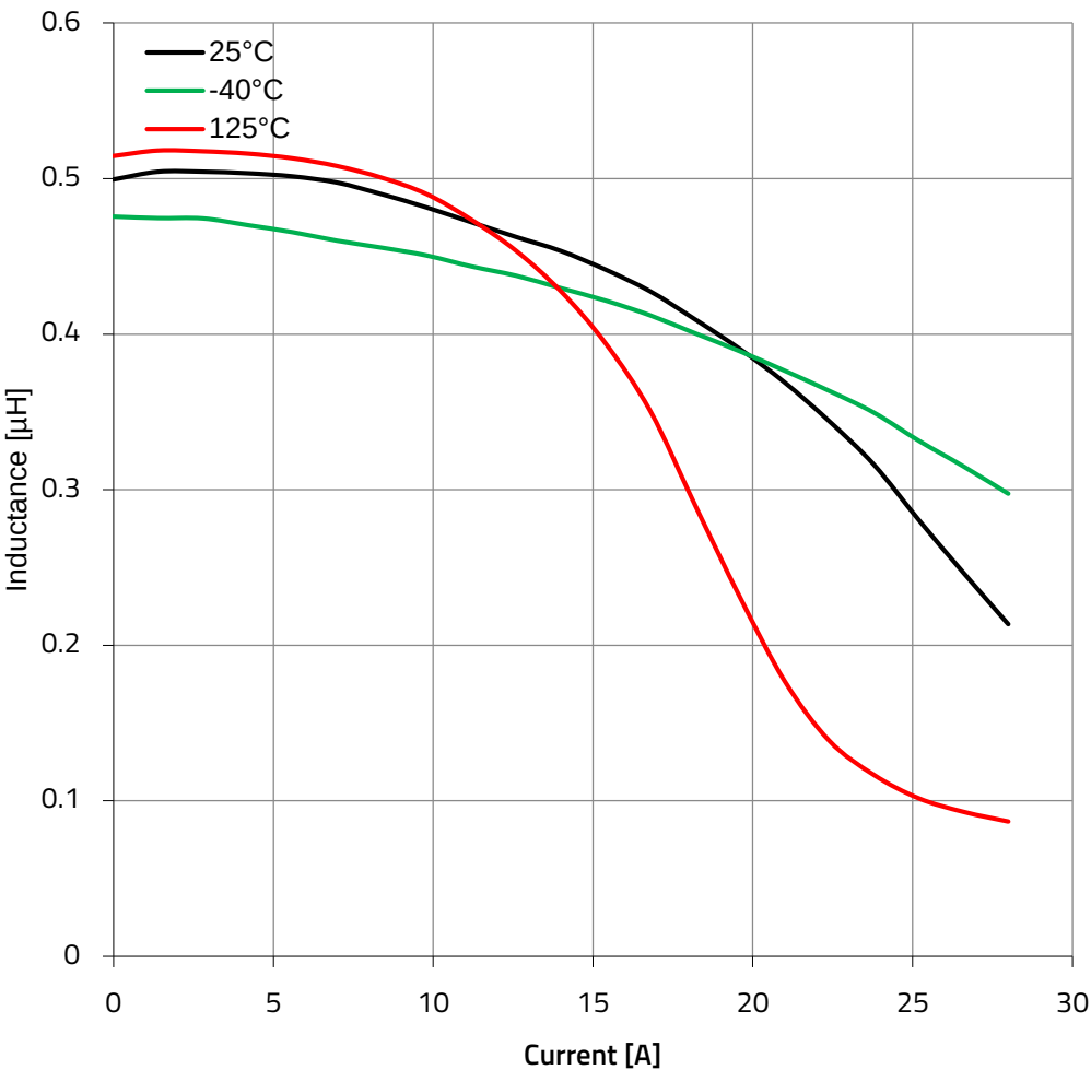
Typical Inductance vs. Current Characteristics - Two Turns:
