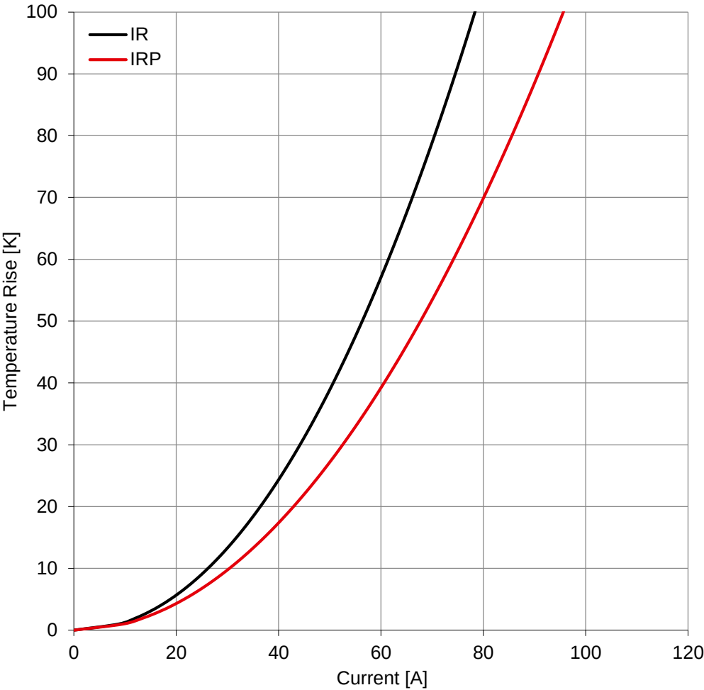
Typical Temperature Rise vs. Current Characteristics - Three Turns:
