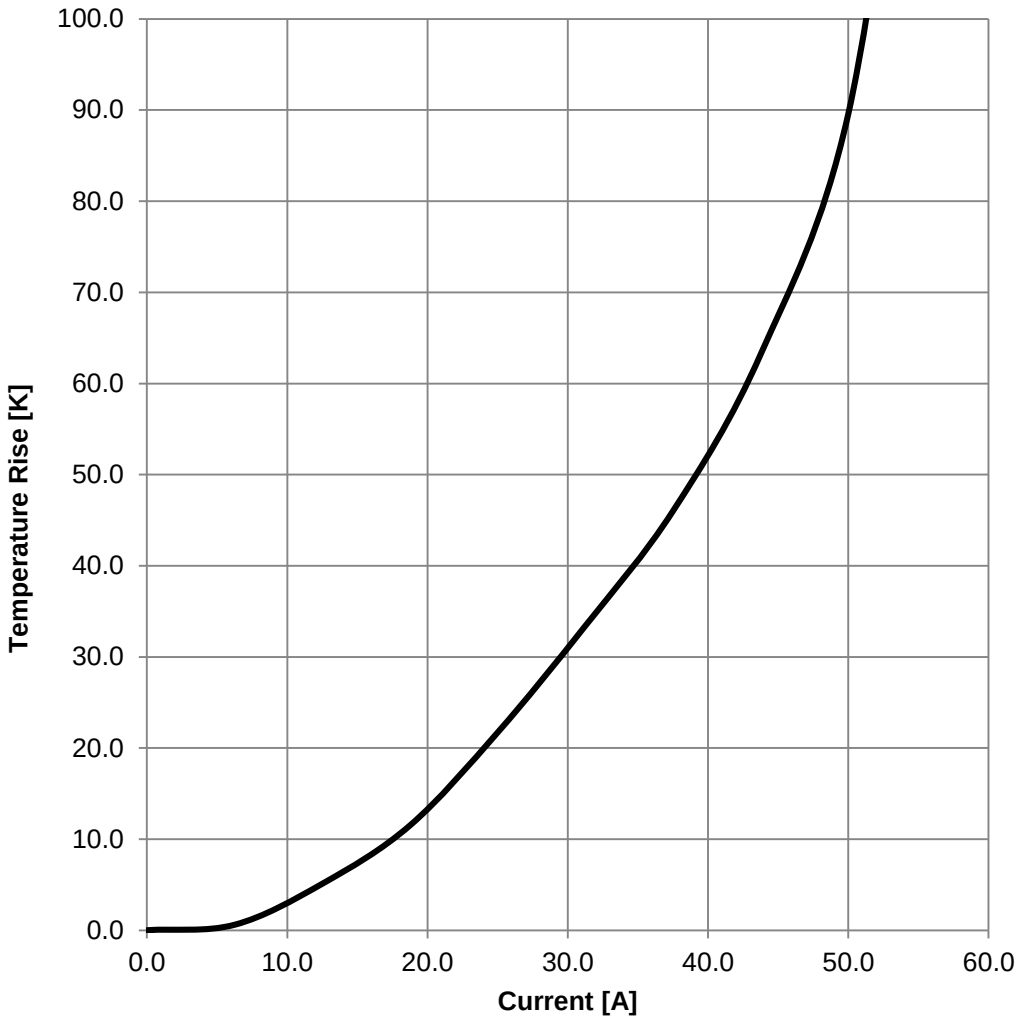
Typical Temperature Rise vs. Current Characteristics - One Turn:
