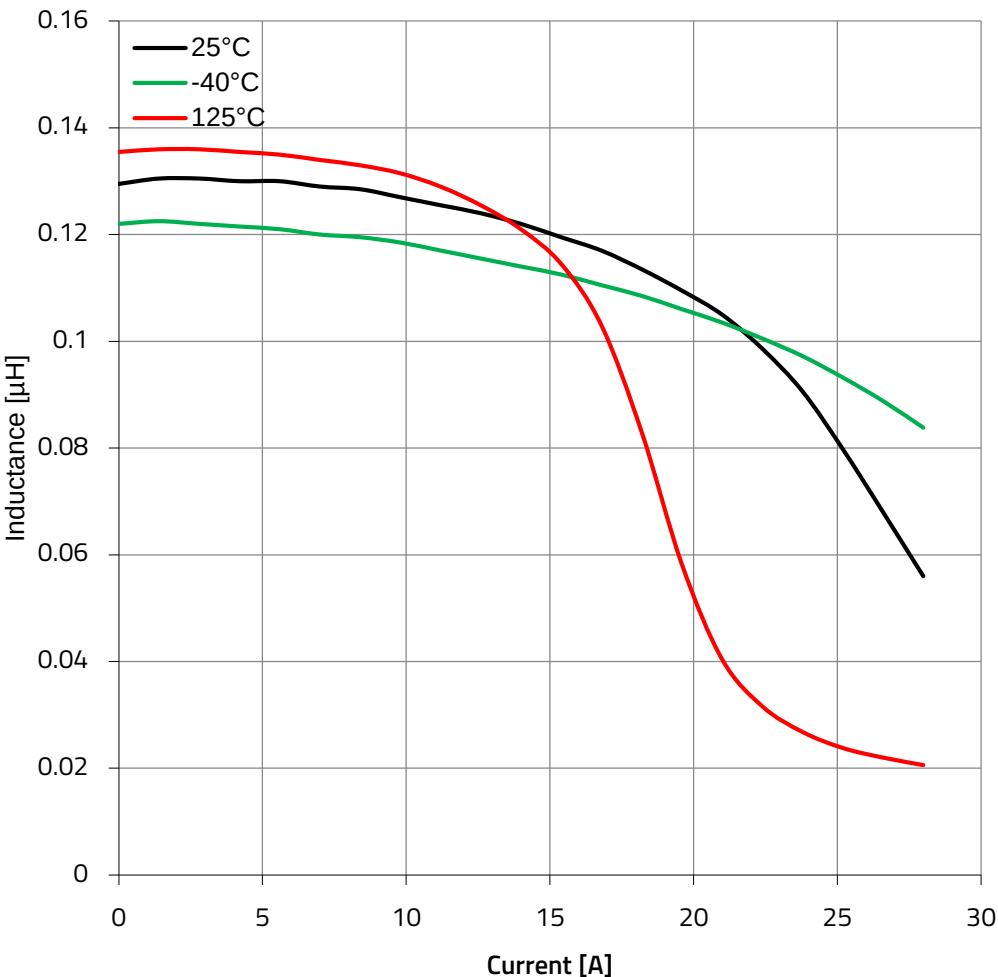
Typical Inductance vs. Current Characteristics - One Turn:
