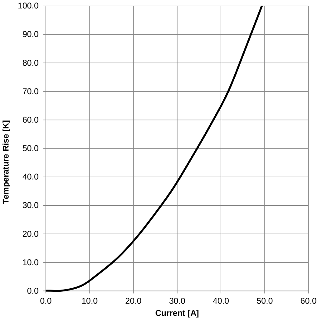
Typical Temperature Rise vs. Current Characteristics - Parallel:
