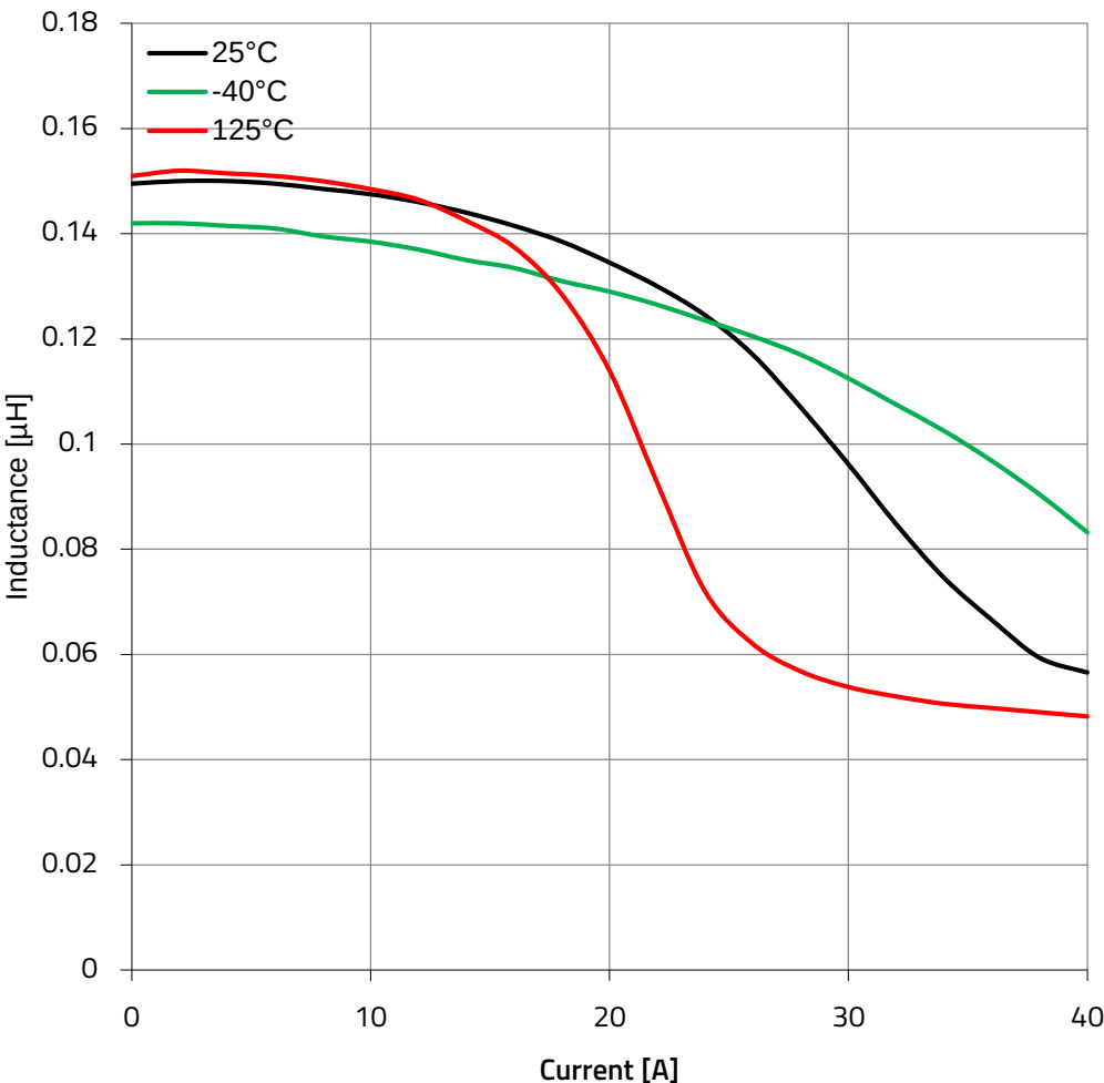
Typical Inductance vs. Current Characteristics - Parallel:
