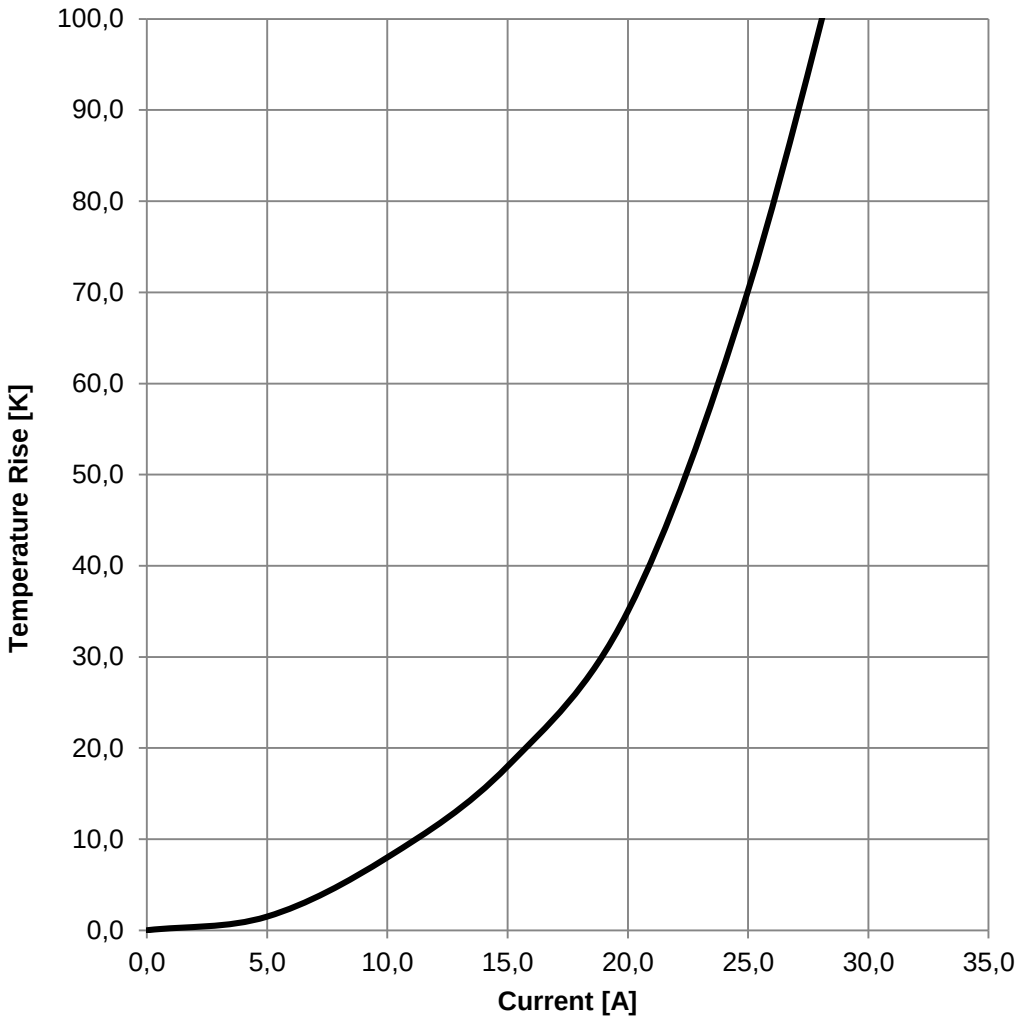
Typical Temperature Rise vs. Current Characteristics - Two Turns:
