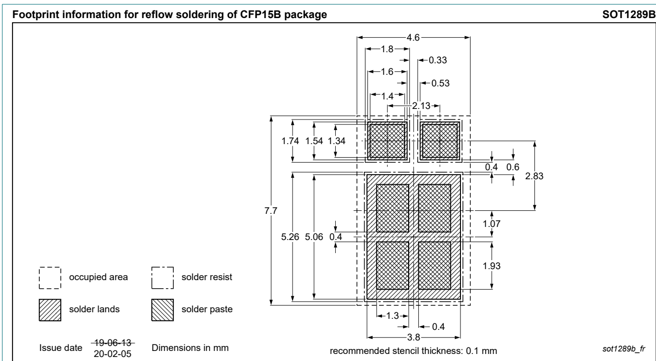
Fig. 19. Reflow soldering footprint for CFP15B (SOT1289B)
