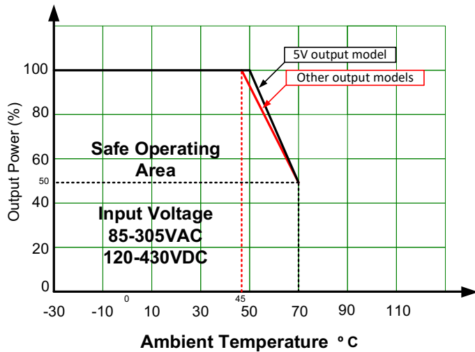
5V model at -30°C to 30°C
