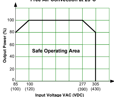
Input derating
