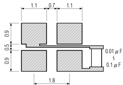
Figure 2) Land Pattern
