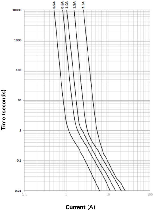
Current vs. time curve 0.5 A to 1.5 A and 2.5 A
