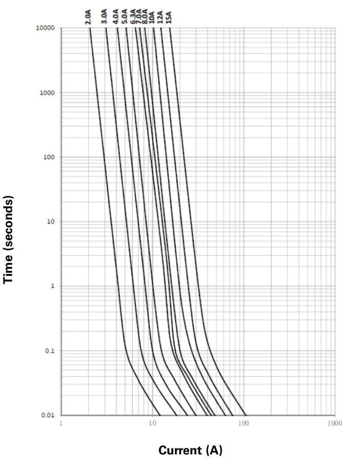
Current vs. time curve 2 A and 3 A and 4 A to 15 A
