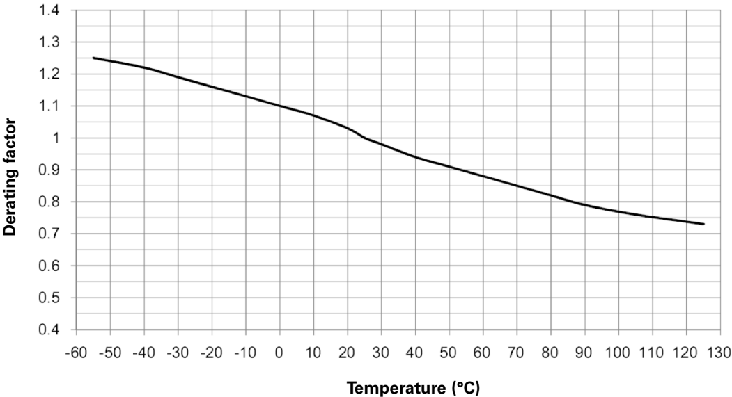
Temperature derating curve
