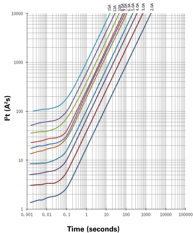
I 2 t vs current curve 2 A and 3 A and 4 A to 15 A
