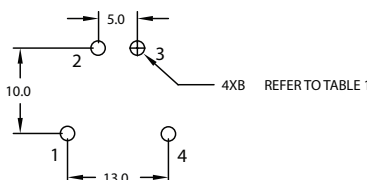
SUGGESTED LAND PATTERN
