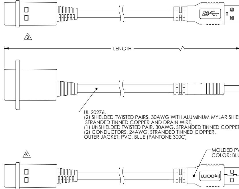
9 PIN USB 3.0 PLUG CONNECTOR
