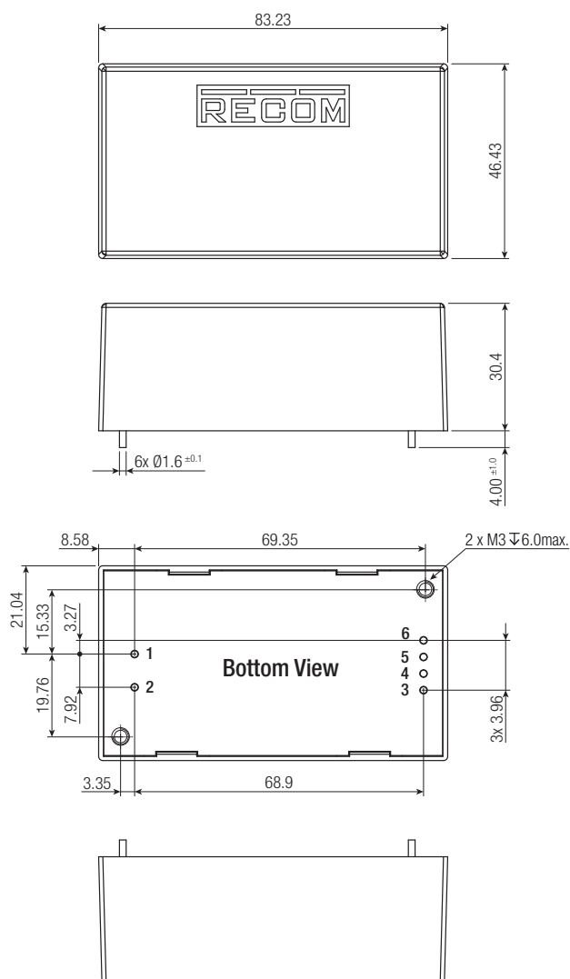
Dimension Drawing (mm)
