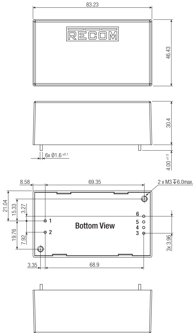
Dimension Drawing (mm)
