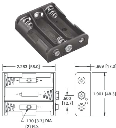
Three (3) Cells - 4.5V
