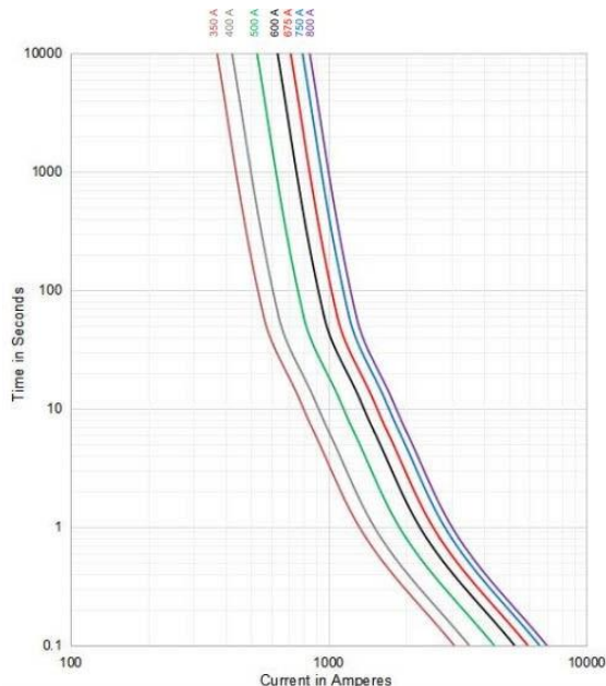
Time Current Curve: 350-800 A
