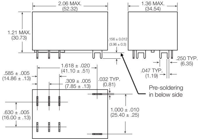
Mounting and termination code 1
