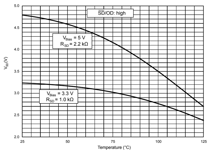
Figure 8. Voltage of \overline{T/SD/OD} pin according to NTC temperature
