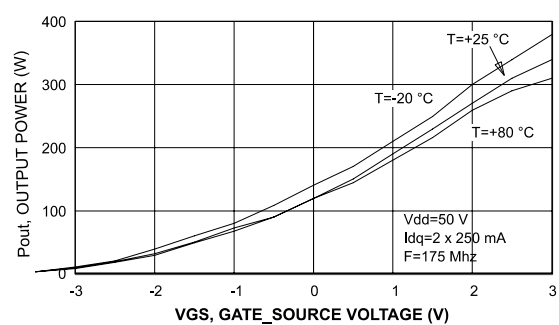
Figure 15: Output power vs. gate voltage
