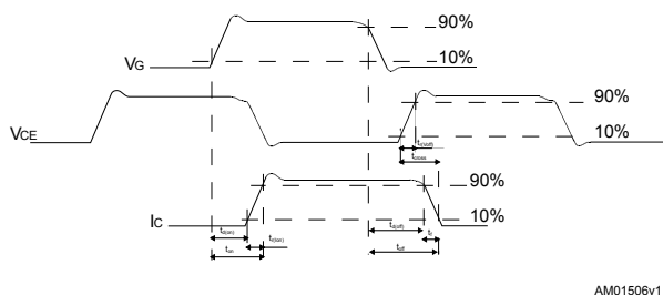
Figure 29. Switching waveform
