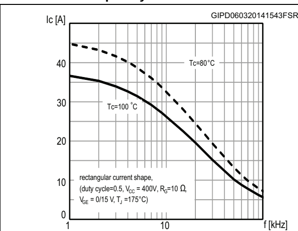
Figure 13. Collector current vs. switching frequency for TO-3PF
