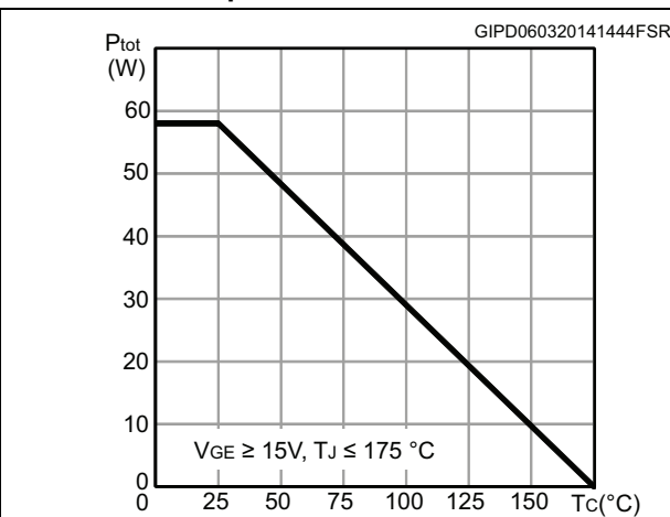
Figure 9. Power dissipation vs. case temperature for TO-3PF
