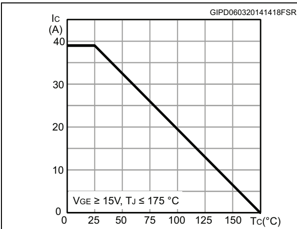
Figure 6. Collector current vs. case temperature for TO-3PF
