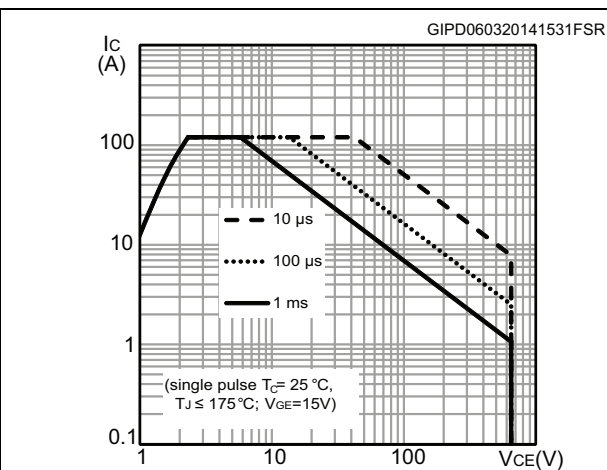
Figure 11. Forward bias safe operating area for TO-3PF
