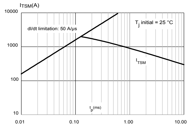
Figure 6. Non-repetitive surge peak on-state current for a sinusoidal pulse ( t_p < 10 ms )
