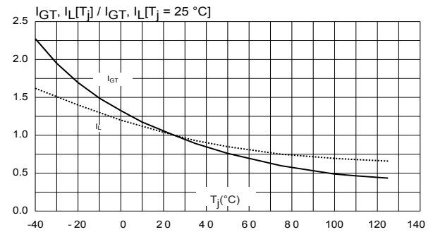
Figure 8. Relative variation of gate trigger current and latching current versus junction temperature (typical values)
