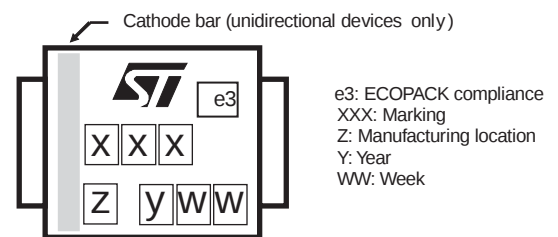
Figure 18: Marking layout
