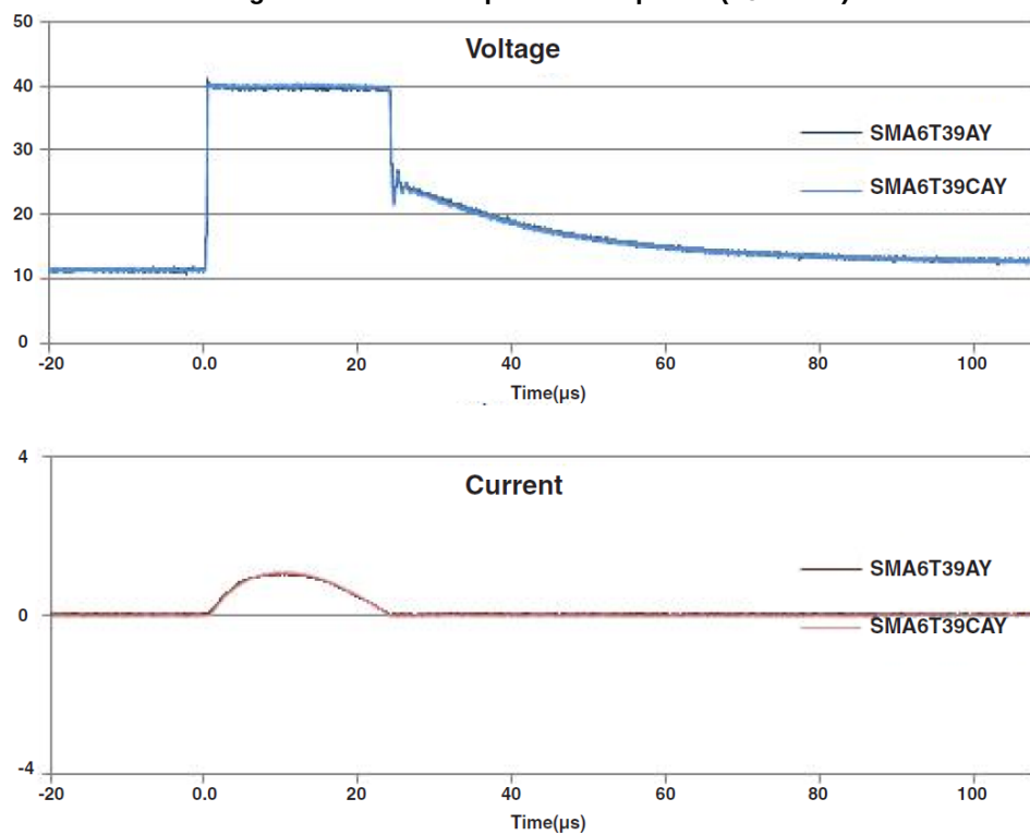
Figure 7: ISO 7637-2 pulse 2a response ( V_s = 50\text{ V} )
