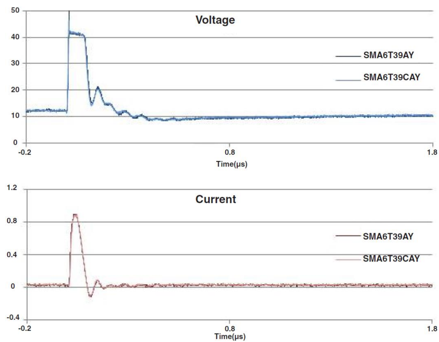
Figure 9: ISO 7637-2 pulse 3b response ( V_s = 100\text{ V} )
