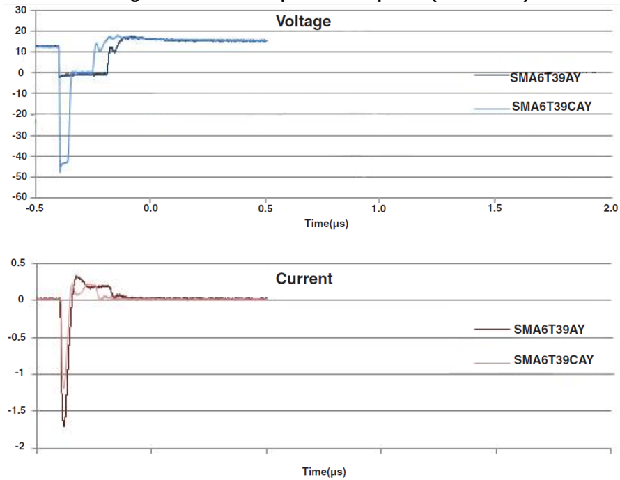
Figure 8: ISO 7637-2 pulse 3a response ( V_s = -150\text{ V} )
