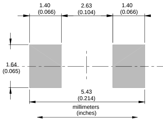
Figure 17: SMA recommended footprint
