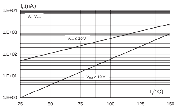
Figure 14: Leakage current versus junction temperature (typical values)
