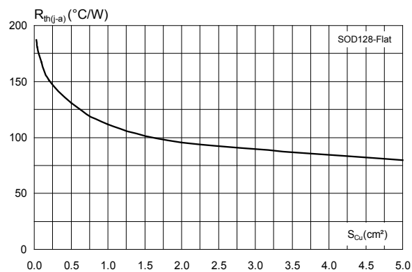
Figure 11. Thermal resistance junction to ambient versus copper surface under each lead (typical values, epoxy printed board FR4, e_{Cu} = 35 μm)
