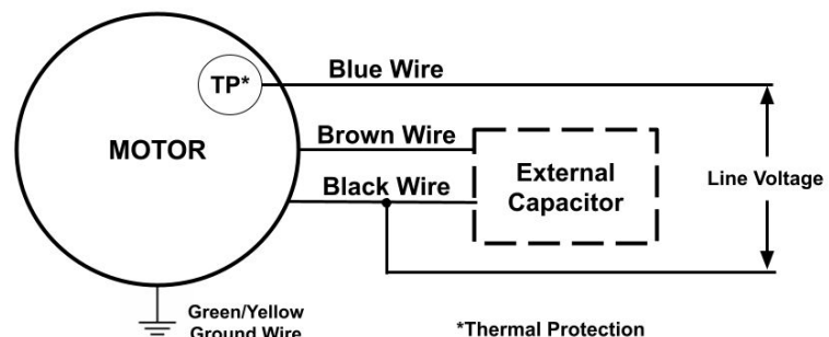
Motor Wiring Diagram
