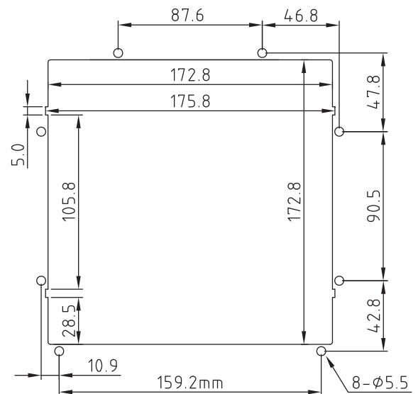
PANEL CUTOUT
