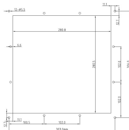
PANEL CUTOUT
