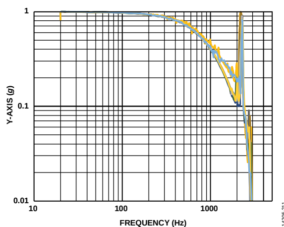
Figure 11. ADXL355 Normalized Frequency Response for Y-Axis at 4 kHz ODR
