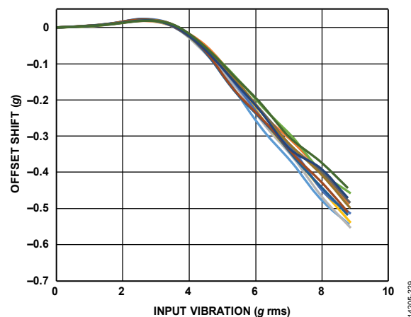
Figure 29. ADXL354 Vibration Rectification Error (VRE), Y-Axis Offset from +1 g, \pm 8 g Range, Y-Axis Orientation = +1 g
