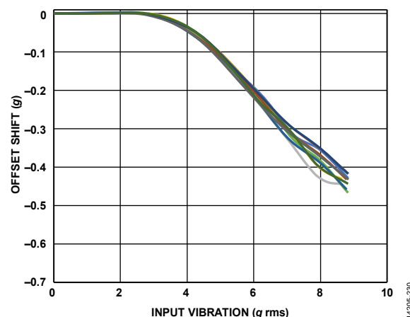
Figure 30. ADXL354 Vibration Rectification Error (VRE), Z-Axis Offset from +1 g, \pm 8 g Range, Z-Axis Orientation = +1 g
