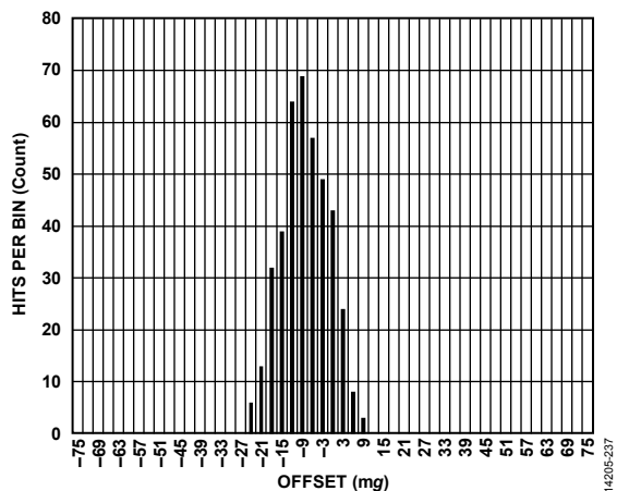
Figure 37. ADXL355 Zero g Offset Histogram at 25°C, X-Axis
