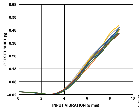
Figure 28. ADXL354 Vibration Rectification Error (VRE), X-Axis Offset from +1 g, \pm 8 g Range, X-Axis Orientation = -1 g
