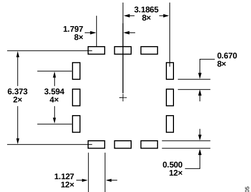
7.2mm x 7.2mm STACKED LGA. ALL DIMENSIONS IN mm.
