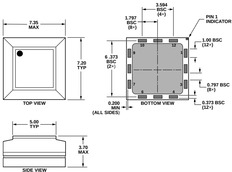
Figure 24. 12-Terminal Land Grid Array [LGA] (CC-12-1)
