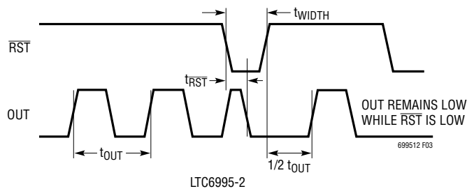
Figure 3. Reset Timing Diagram (POL Bit = 0)
