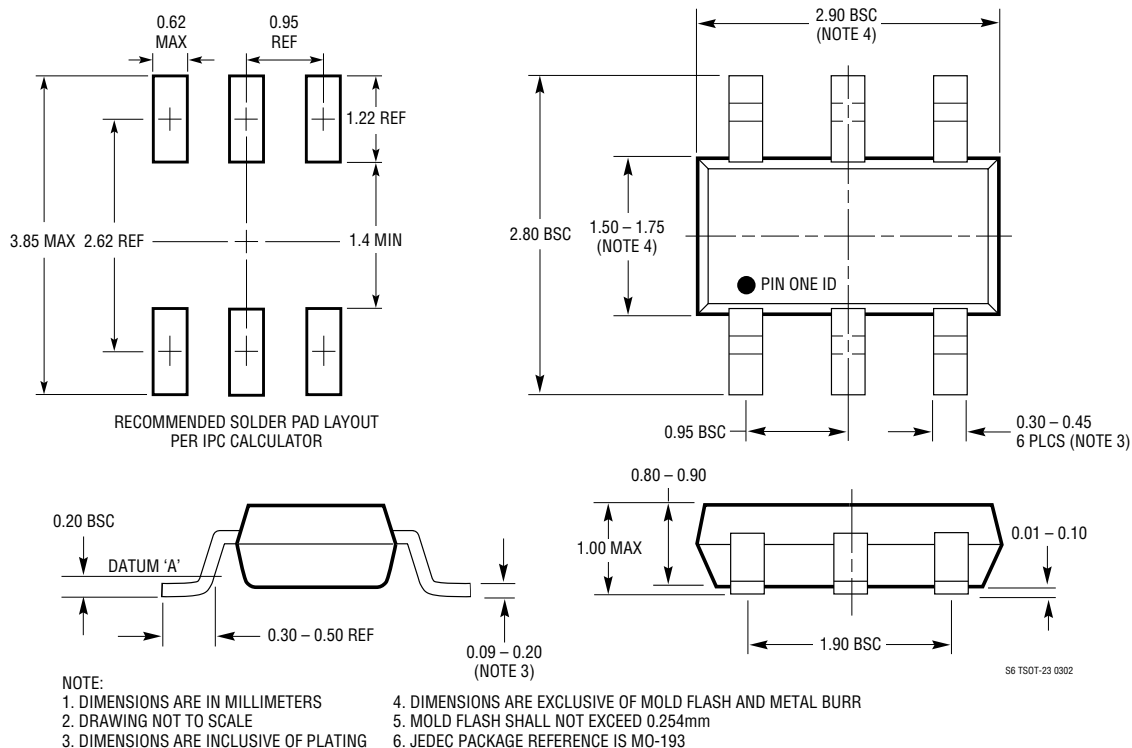
S6 Package 6-Lead Plastic TSOT-23 (Reference LTC DWG # 05-08-1636)
