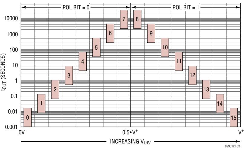
Figure 2. Frequency Range and POL Bit vs DIVCODE
