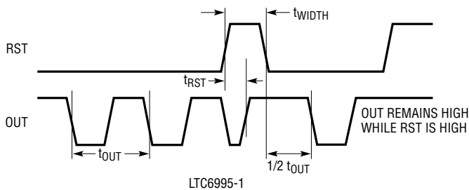
Figure 4. Reset Timing Diagram (POL Bit = 1)
