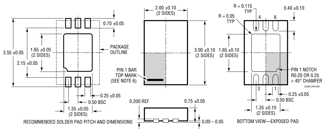
DCB Package 6-Lead Plastic DFN (2mm × 3mm) (Reference LTC DWG # 05-08-1715 Rev A)
