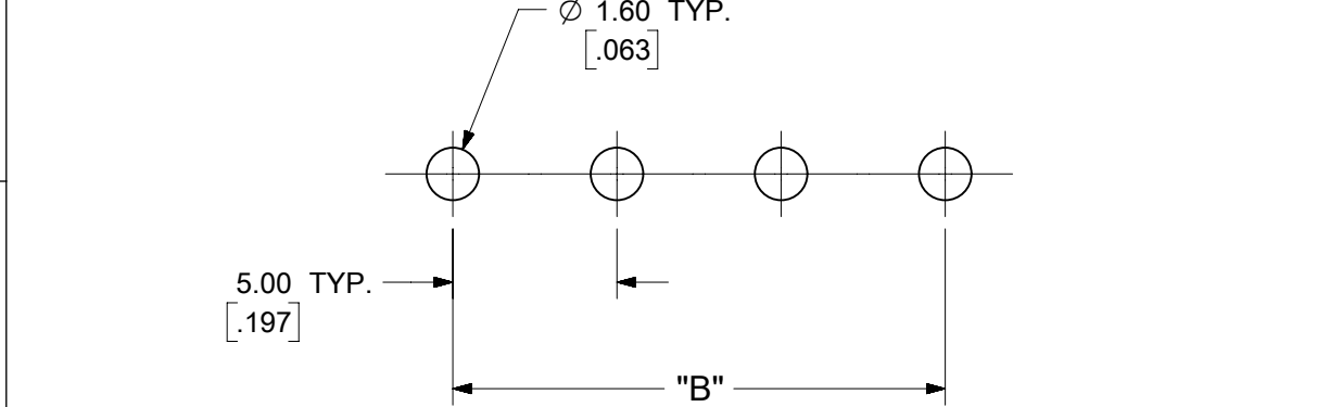
PCB LAYOUT
